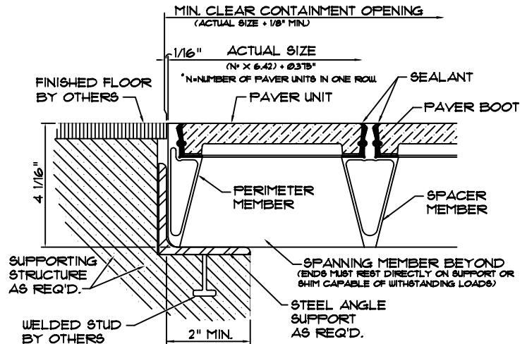
FLOOR SECTION INTERIOR INSTALLATION SCALE: NONE
